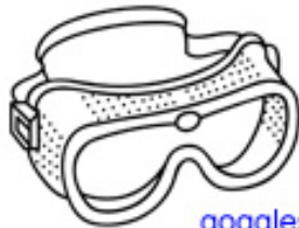
goggles
