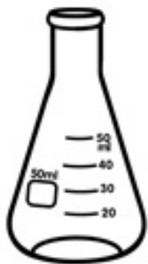
flask
