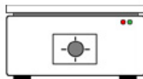
hot plate
