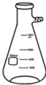
side-arm flask
