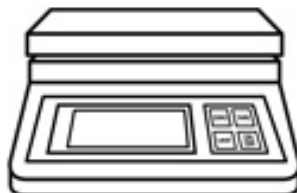
electronic balance
