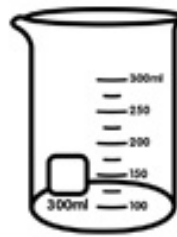
beaker
